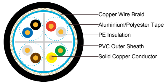
SF/UTP CAT6
