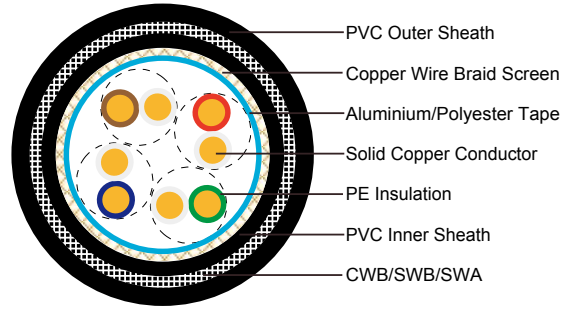
SF/UTP CAT6
